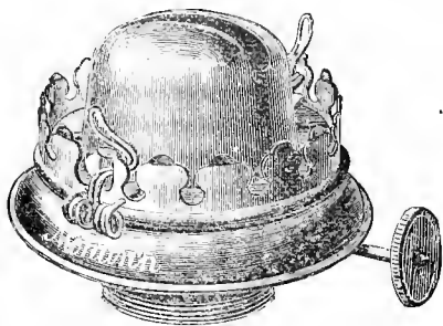
Fig. 3376. "MONARCH" BURNER ( \frac{2}{3} full size). (Nos. 2, 3 and 18 Chimneys.)
